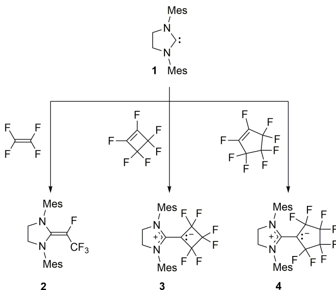
Scheme 2. Addition of fluoro-olefins to 1 yields adducts 2-4 .
