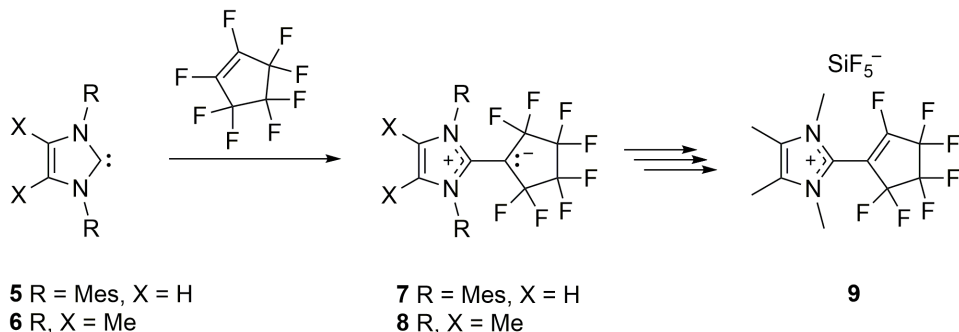
Scheme 4. Addition of fluoro-olefins to unsaturated imidazol-2-ylidenes ( 5 , 6 ) yields adducts 7 and 8 . Further decomposition of 8 is observed to 9 .
