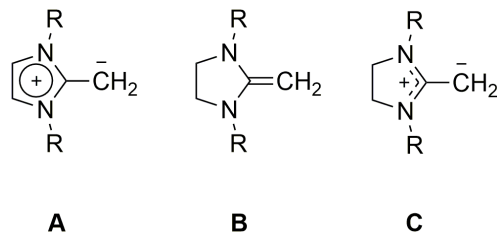
Scheme 1. 2-Methyleneimidazol(in)es are represented as resonance structures A-C .
