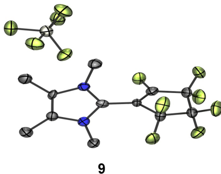
Figure 2. X-ray crystal structure of 9 . Thermal ellipsoids drawn at the 50% probability level.
